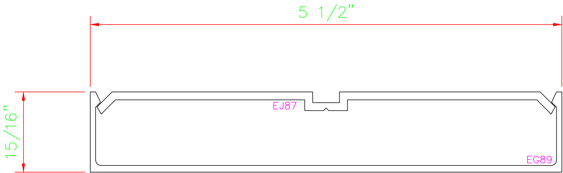
EG89 / EJ87 5 1/2" X 15/16" MULLION COVER & CLIP
